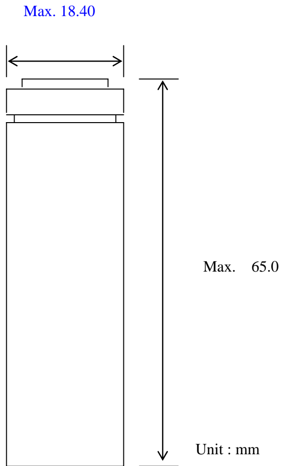
Fig.1. Outline Dimensions of ICR18650-24E
